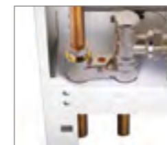
Accommodated within the casing, the Stelrad LST i Plus Deco emitter, with TBSE valve arrangement and 2 x 1/2" BSP connections as standard.
