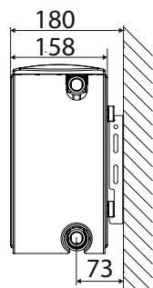
SIDE ELEVATION
