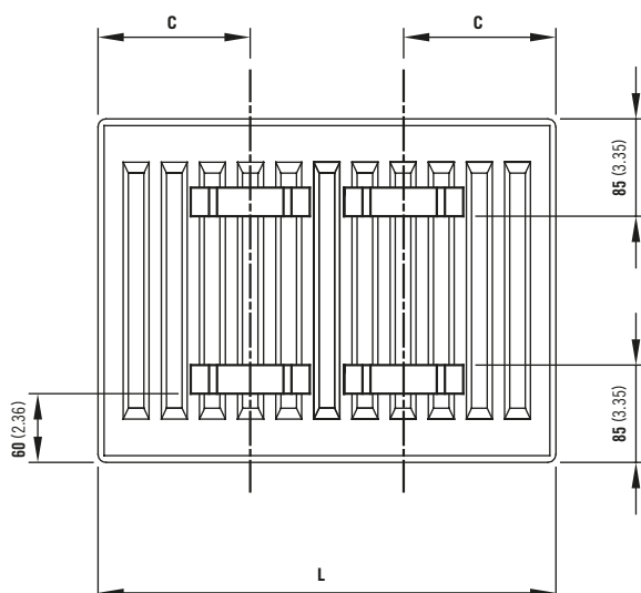
REAR ELEVATION
