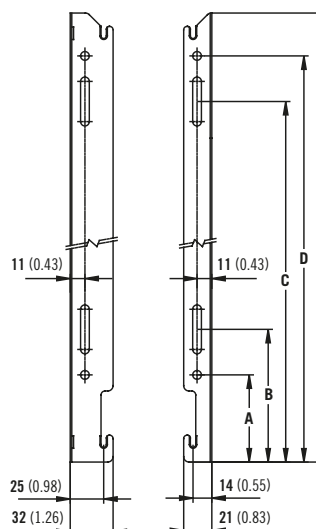
K1, P+ and K2 (OVER 300mm)
