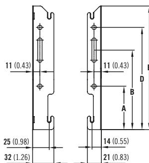
K1, P+ and K2 (300mm)
