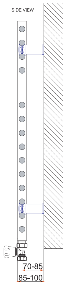
MOUNTING BRACKET ILLUSTRATION 4 pcs UNIVERSAL MOUNTING BRACKET
